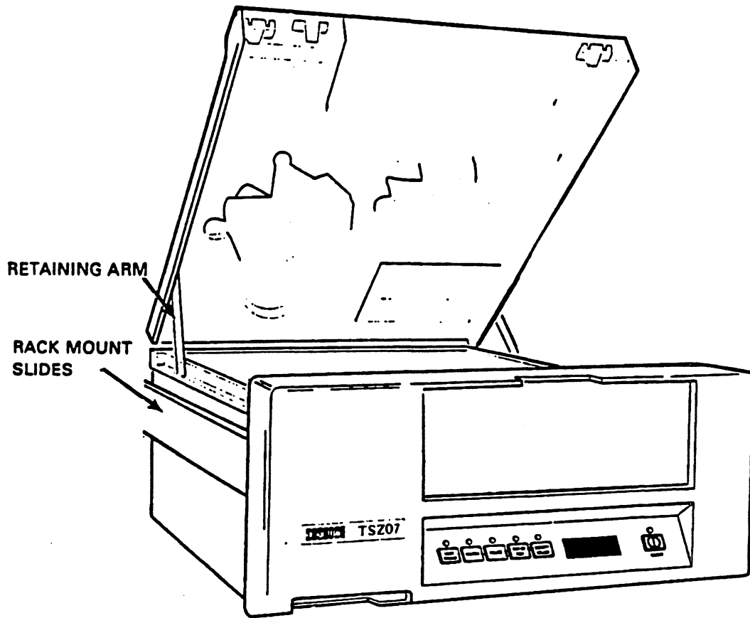
Figure 2-15: TSZ07 Cover Retaining Arm - Rackmount Model
