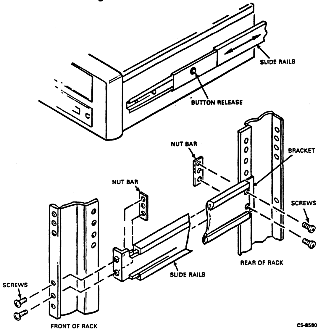
Figure 2-16: Rack Mounting the TSZ07
