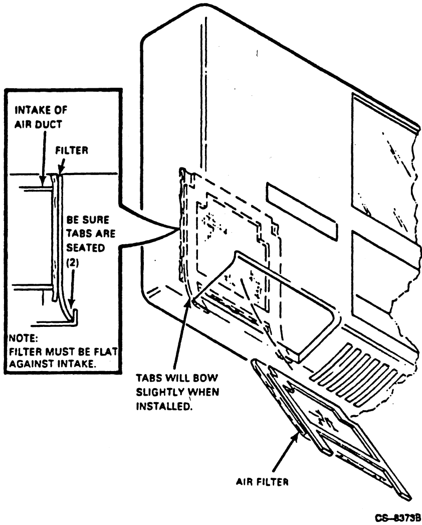
Figure 4-2: Air Filter
