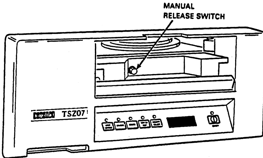
Figure 3-4: Location of the Manual Release Switch
