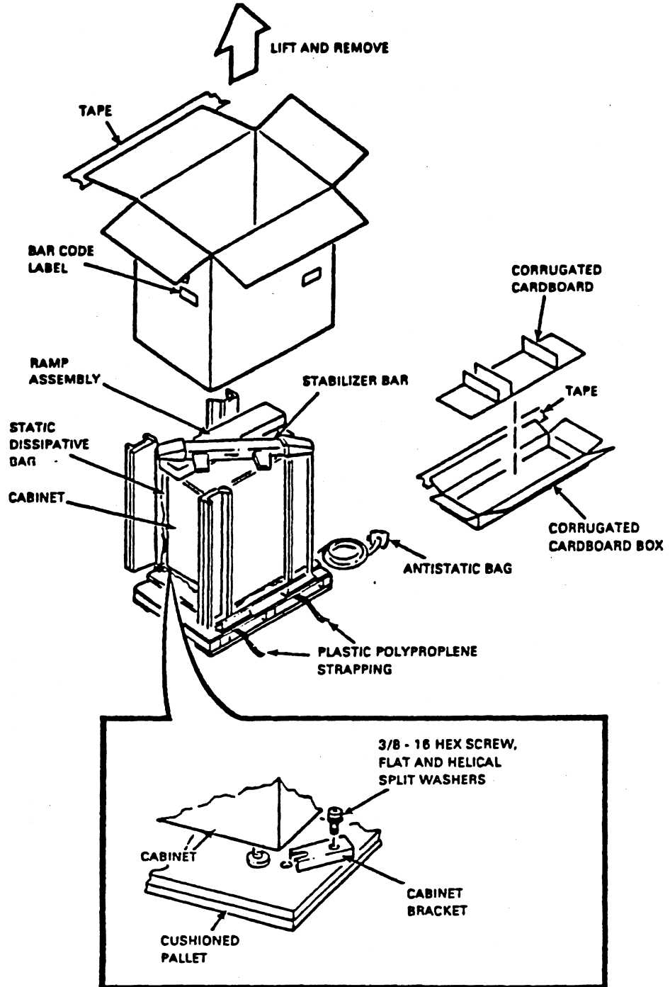
Figure 2-7: Cabinet Carton Removal
