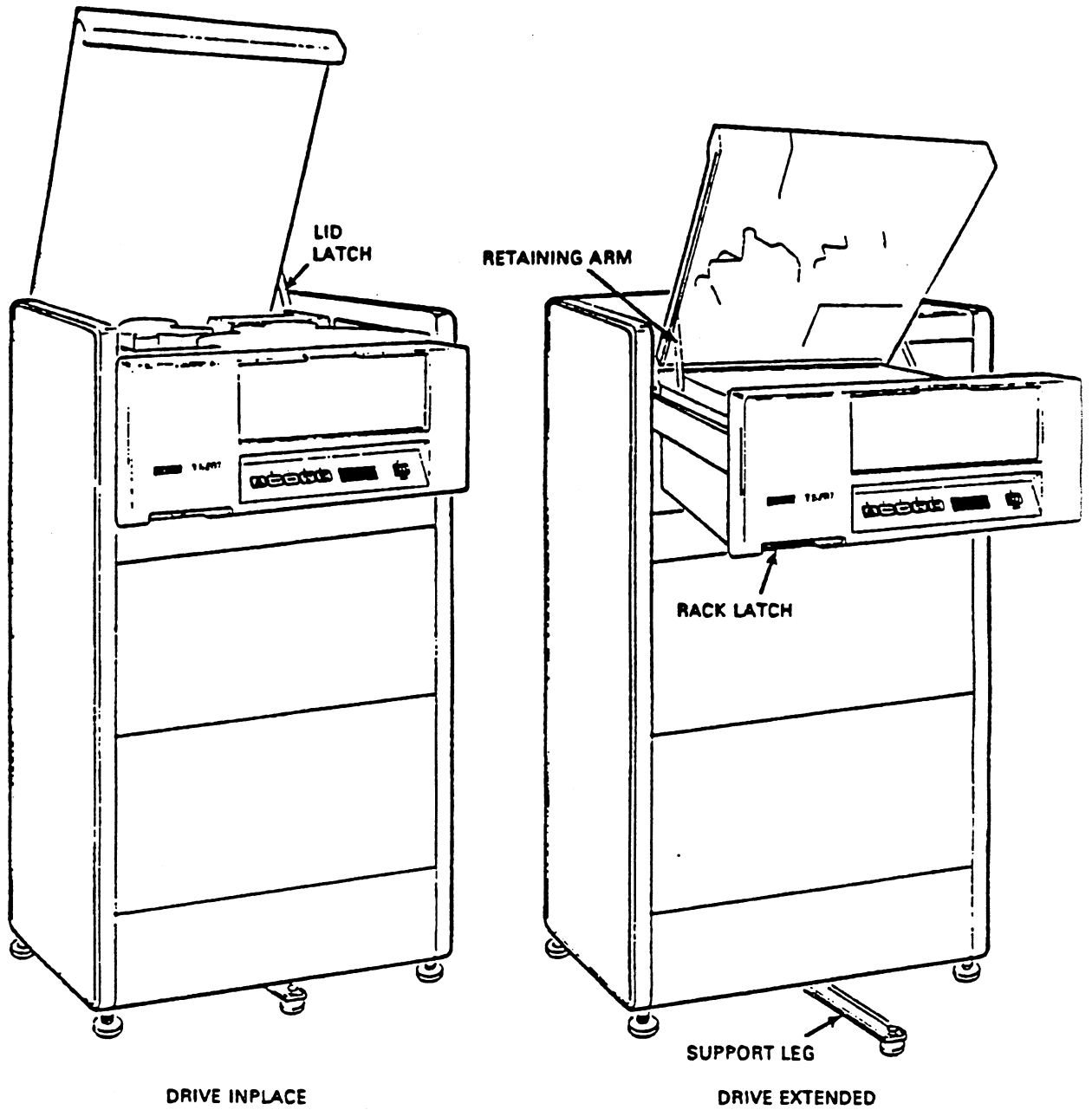
Figure 2-14: Opening Cabinet Lid
