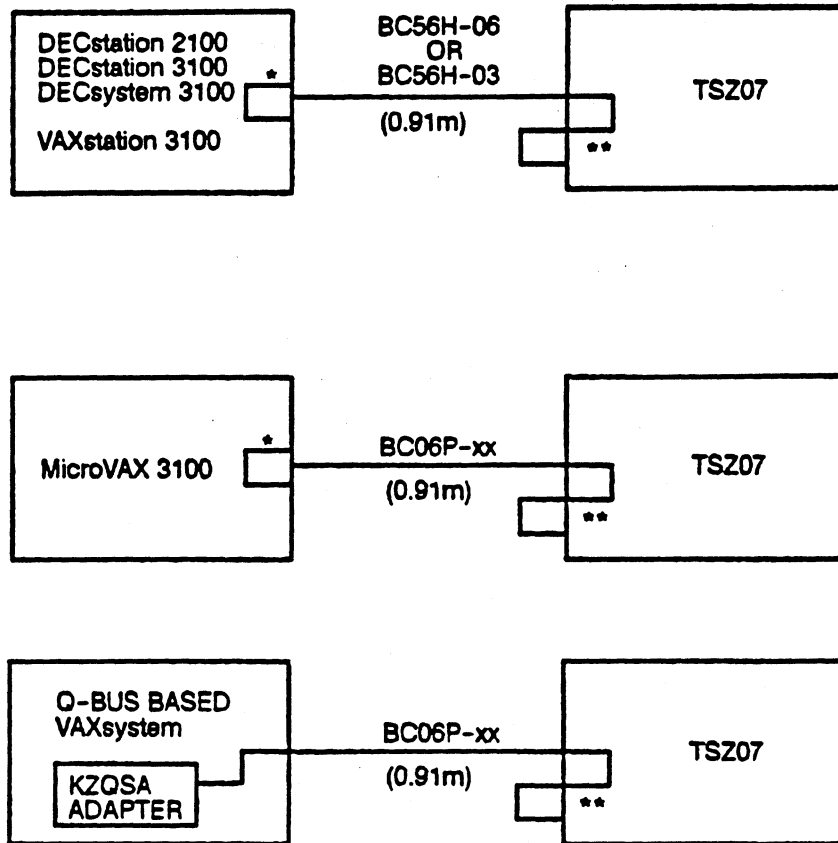
Figure 2-5: Typical Standalone SCSI Configurations
