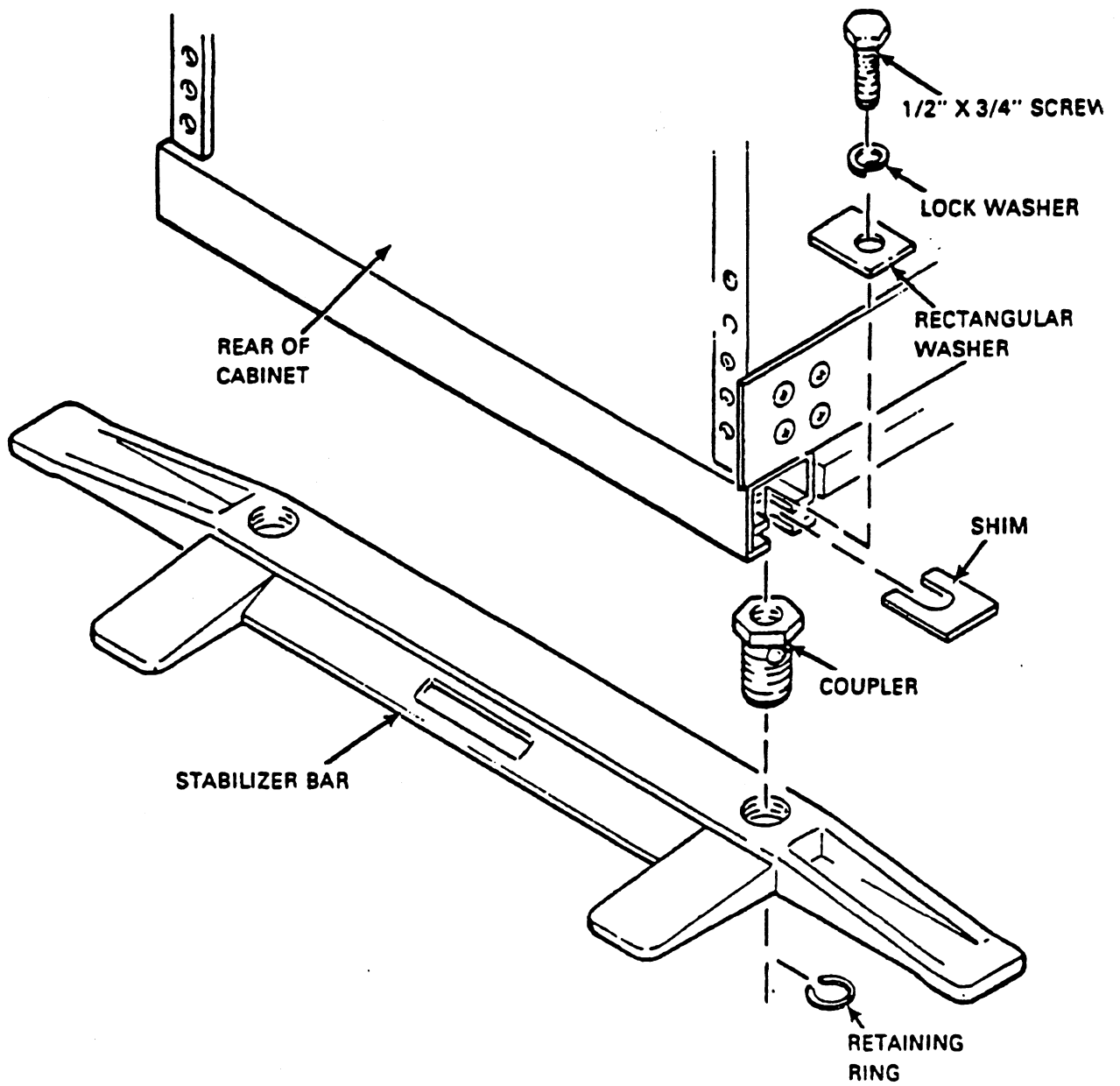
Figure 2-13: Installing the Cabinet Stabilizer
